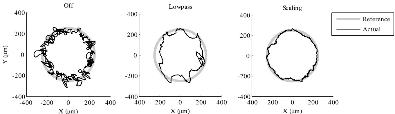
Fig. 33. Effect of cancellation on 2D tip motion. These are typical results from three different circle tracing tasks (approximately 15 seconds each circle).
