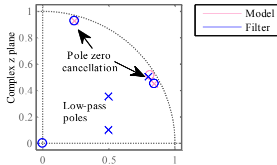
Fig. 22. Structure of Q_l(z) (inverse filter for the lateral mode), compared to manipulator model. Low-frequency resonances are approximately canceled, while a low-pass filter ensures a robust high-frequency gain margin.
