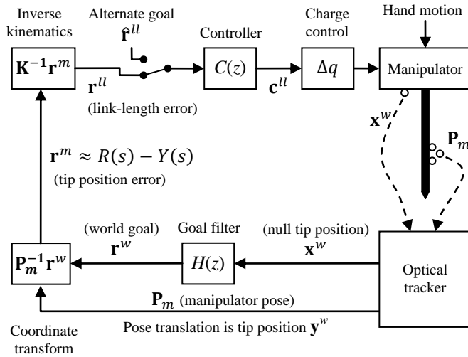
Fig. 15. Control system with kinematics, showing the coordinate transforms that implement the 3D signal flow. The optical tracker measures both the system input (hand motion \mathbf{x}^w ) and the output (manipulator pose \mathbf{P}_m ). Inversion of the pose creates negative feedback that forces the tip to track \mathbf{r}^w (an estimate of the voluntary motion).
