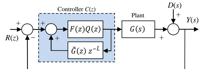
Fig. 18. Block diagram equivalent to Fig. 17 drawn with unity negative feedback, showing similarity to PID and other conventional controllers.
