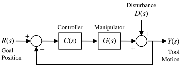
Fig. 11. Position servo loop small-signal model with disturbance. This servo loop stabilizes the tip position without any direct measurement of hand motion, canceling disturbance from any source.
