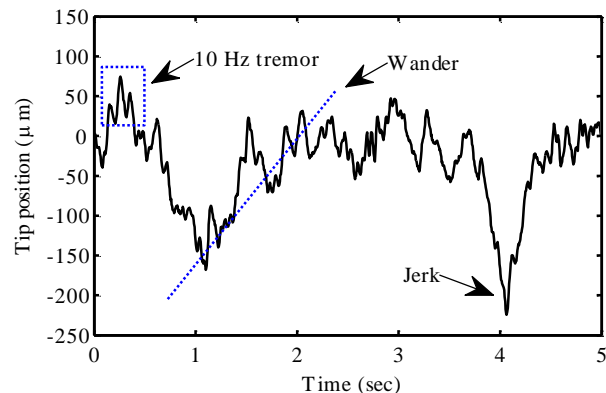
Fig. 1. Tremor signal with identified features. Low-frequency wander and non-periodic jerk components dominate the peak-to-peak amplitude.
