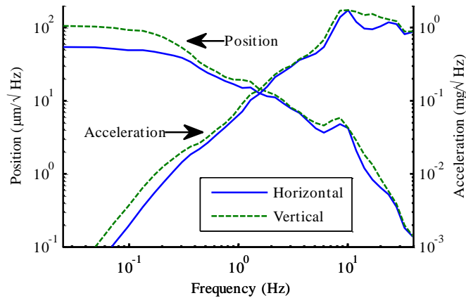
Fig. 2. Spectra of position error and acceleration during “hold still” task. The acceleration spectrum shows a 10 Hz tremor peak, yet in the position spectrum, low-frequency error dwarfs this 10 Hz peak, leveling off in the band where visual feedback is effective. In this visual feedback band, error is greater in the vertical (visual depth) direction.
