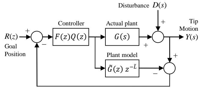
Fig. 17. Internal Model Control architecture. The actual plant and the model receive the same command. The difference of the measured and predicted positions (disturbance or modeling error) is fed back to the input.
