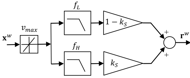
Fig. 13. Cancellation filter structure. This implements the shelving response of the scaling algorithm, and also limits the goal velocity.
