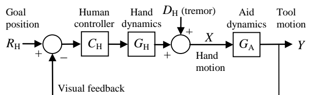
Fig. 4. Simple feedback model of the human-in-the-loop system with a manipulation aid. Tremor is modeled as a disturbance D_H added to the hand motion. Eye-hand feedback acts to minimize the effect of this disturbance. G_A is the dynamic contribution of the aid system, which may destabilize the overall eye-hand feedback.
