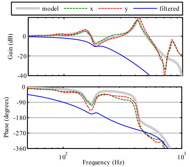
Fig. 21. Manipulator x and y frequency response data, shown superimposed on \tilde{G}_l(z) , the lateral response model. Filtered is Q_l \tilde{G}_l , the designed frequency response including the effect of the lateral inverse filter. This lowpass response robustly suppresses high-frequency resonances, but adds phase lag.
