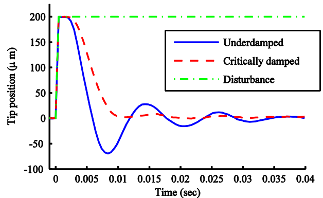
Fig. 26. Detail of initial transient in response to handle position step. The disturbance is injected numerically, so the rise-time is one sample period. The critically damped tuning has hardly any overshoot, but is slower in bringing the tip back to zero (less bandwidth).
