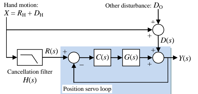
Fig. 12. Micron small-signal model with cancellation filter. Hand motion is a combination of the desired motion R_H and tremor D_H (see Fig. 4). This motion is measured and filtered to establish the goal position so that voluntary motion is possible. The position servo loop is from Fig. 11.
