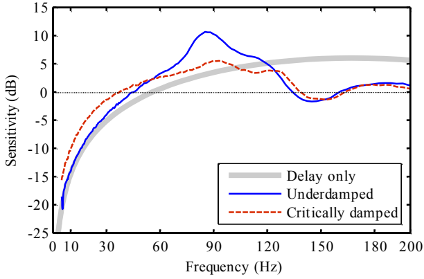
Fig. 23. High-frequency motion disturbance rejection (sensitivity) for both control tunings. “Delay only” is a theoretical limit. Inevitably disturbance is magnified at high frequencies, but this is harmless because tremor disturbance drops off above 10 Hz (Fig. 2). Note linear frequency scale.
