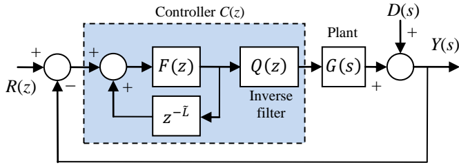
Fig. 19. IMC architecture simplification possible when Q = \tilde{G}^{-1} , giving a lead-lag controller with approximate inversion of plant dynamics.
